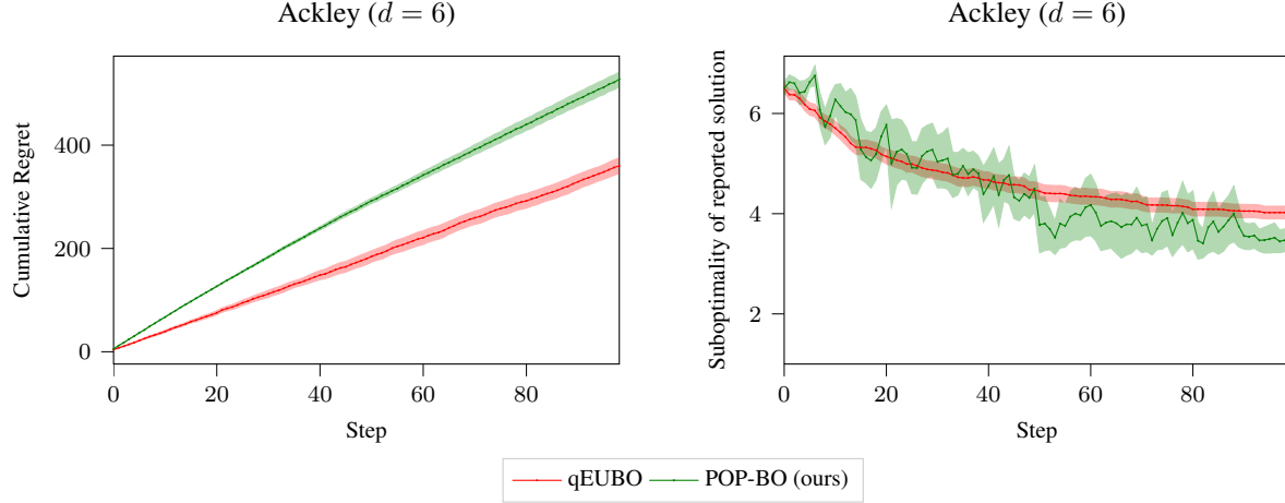
Figure 6. Cumulative regret and the suboptimality of the reported solution for the 6-dimensional Ackley function optimization problem, where the shaded areas represent \pm 0.5 standard deviation.
