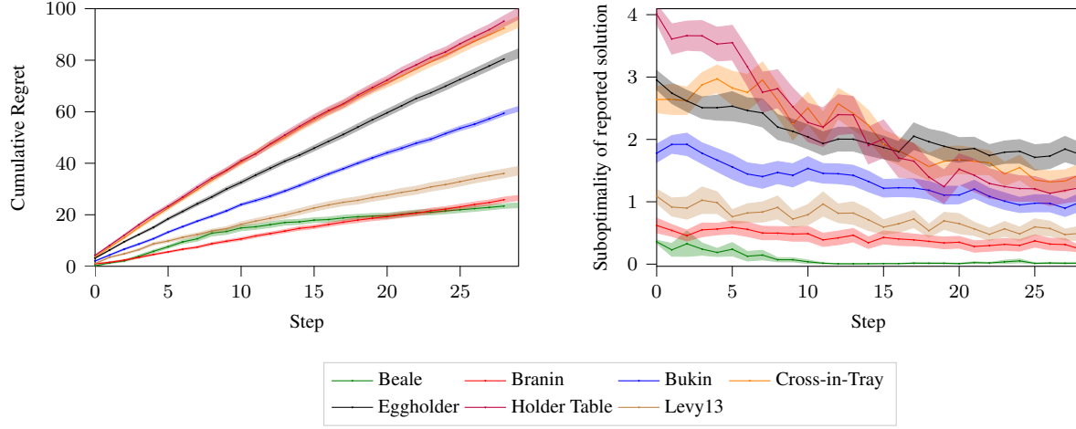
Figure 9. Cumulative regret and the suboptimality of the reported solution of POP-BO algorithm for the different test problems in Tab. 2.
